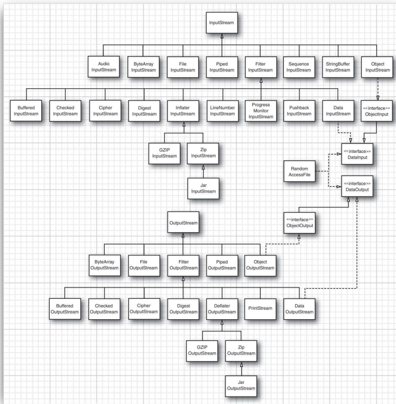
Figure 2.1 Input and output stream hierarchy
